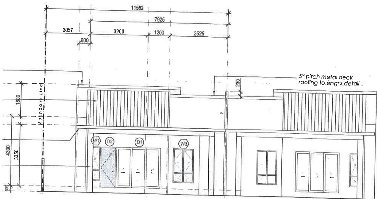
PANDANGAN HADAPAN
