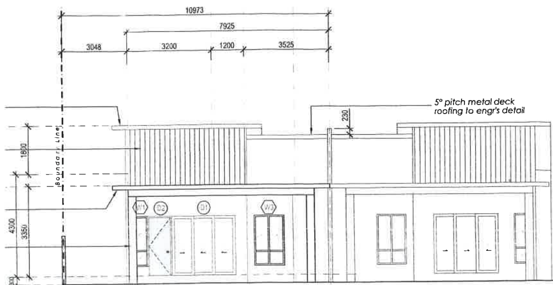
PANDANGAN HADAPAN
