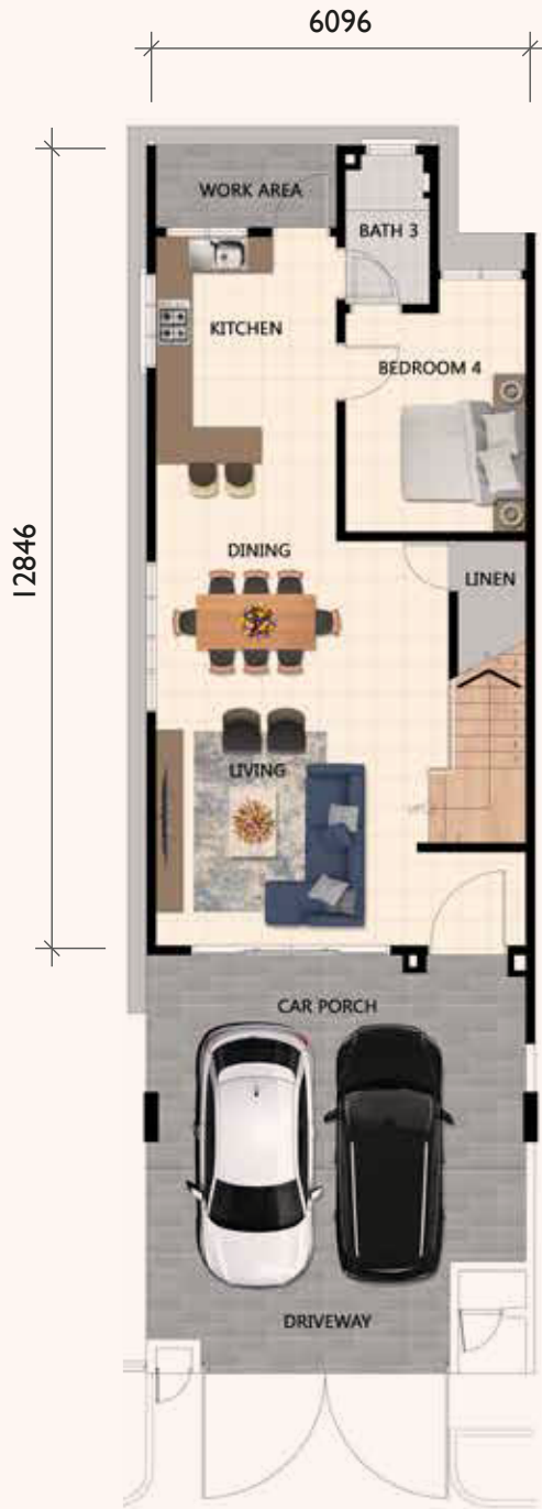
GROUND FLOOR
