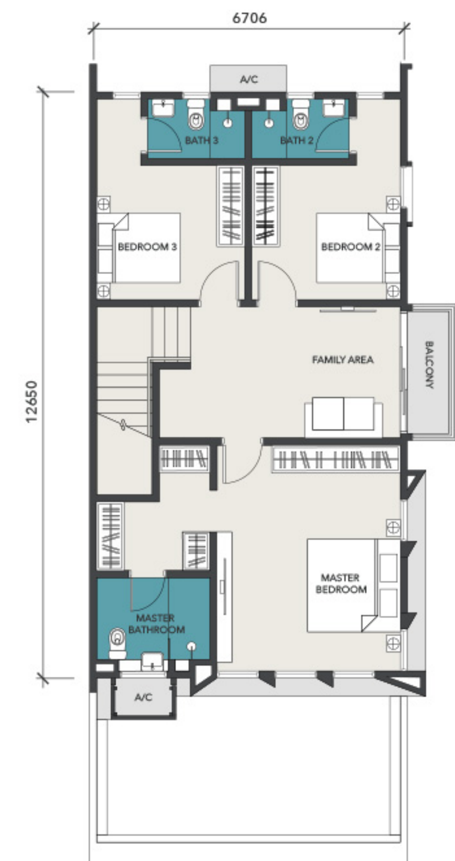
FIRST FLOOR
