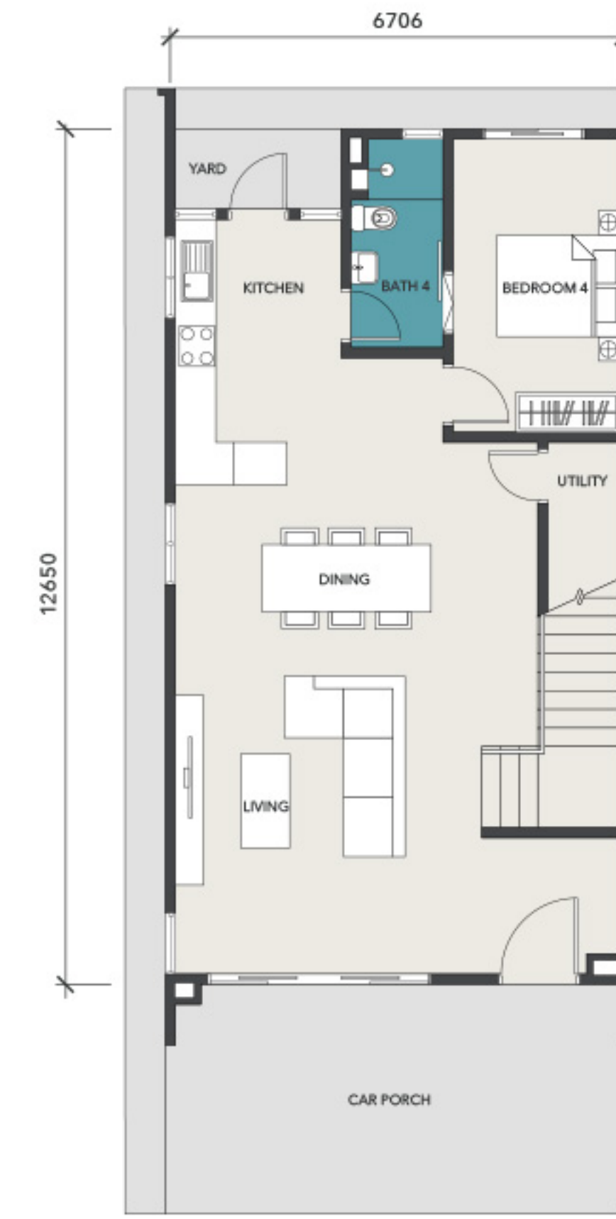
GROUND FLOOR
