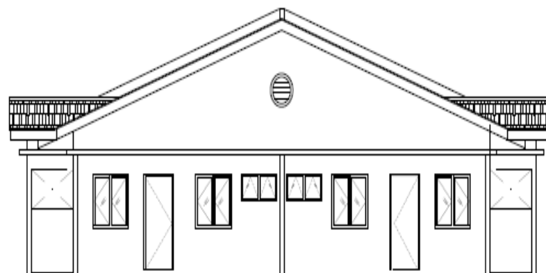
PANDANGAN HADAPAN
