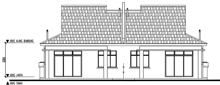
PANDANGAN HADAPAN
