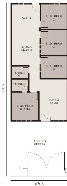
TERES B (22'X66')
