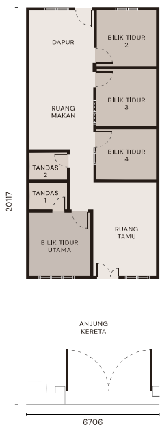
TERES A (22'X70')
