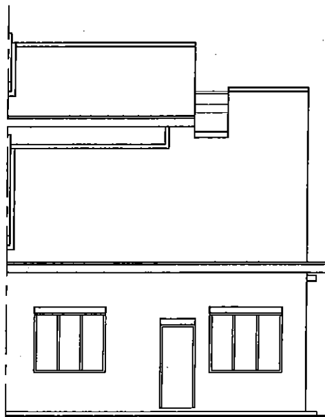
PANDANGAN HADAPAN
