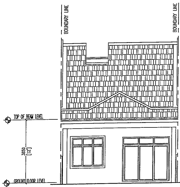
PANDANGAN HADAPAN
