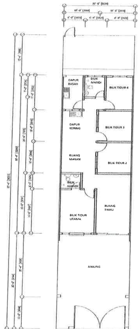
LOT 1411 - PELAN LANTAI
