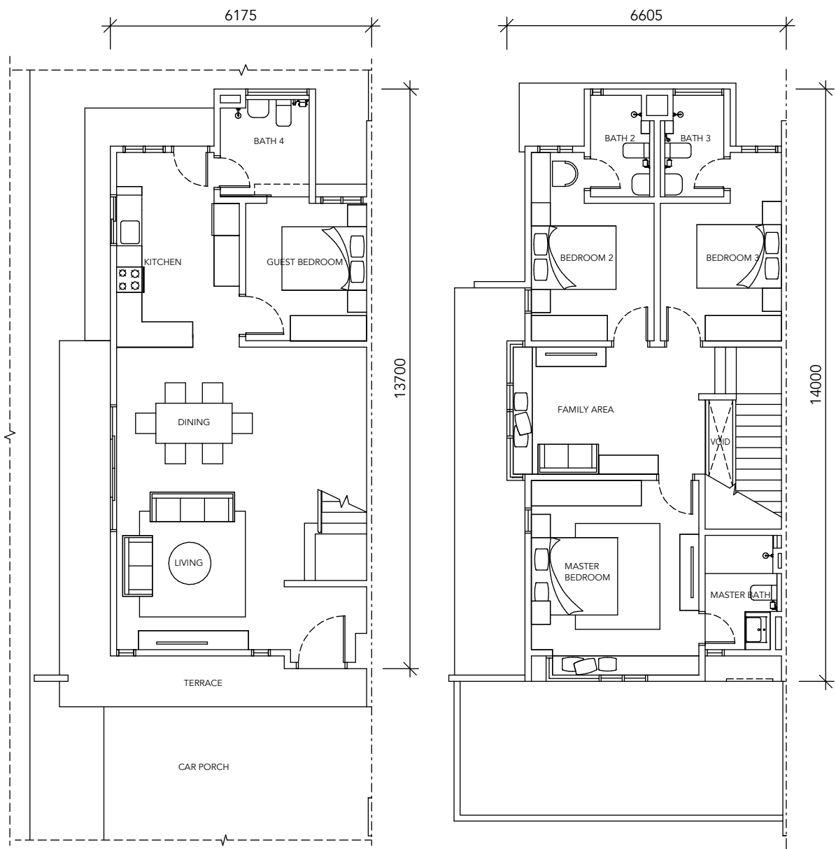
Ground Floor
