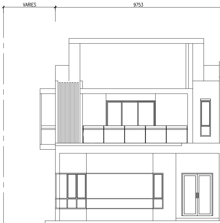
PANDANGAN HADAPAN
