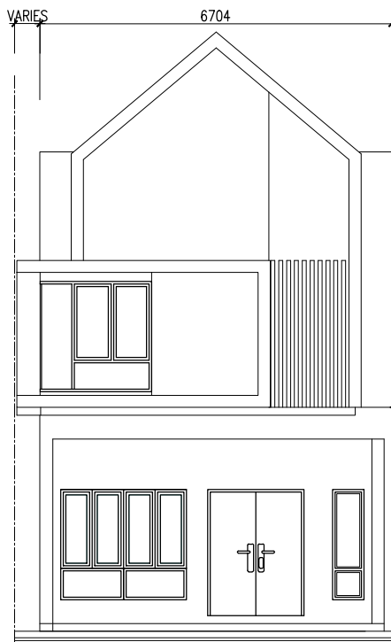
PANDANGAN HADAPAN
