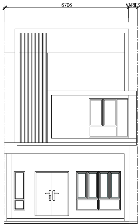
PANDANGAN HADAPAN
