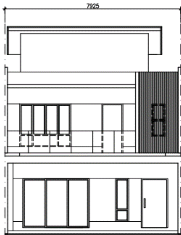
PANDANGAN HADAPAN
