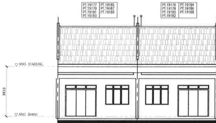
PANDANGAN HADAPAN
