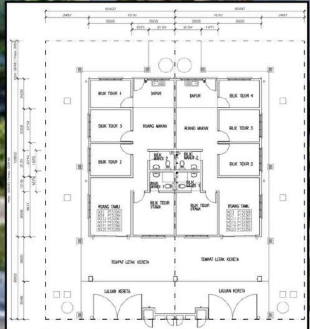
Type A1 - 33.7' x 74'
