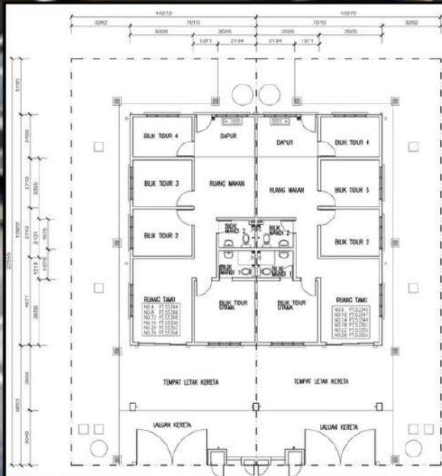
Type A1 - 34.44' x 74'
