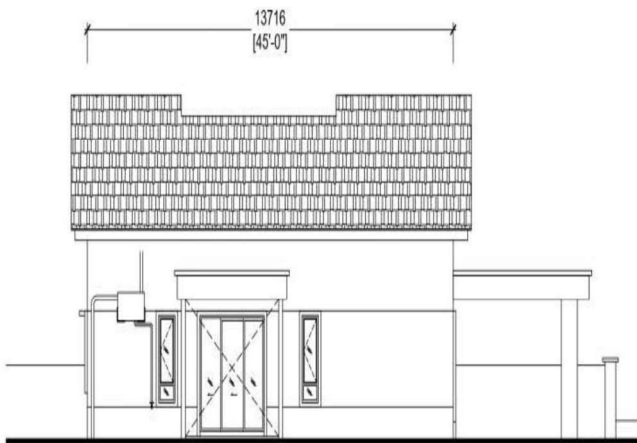
Pandangan Hadapan
