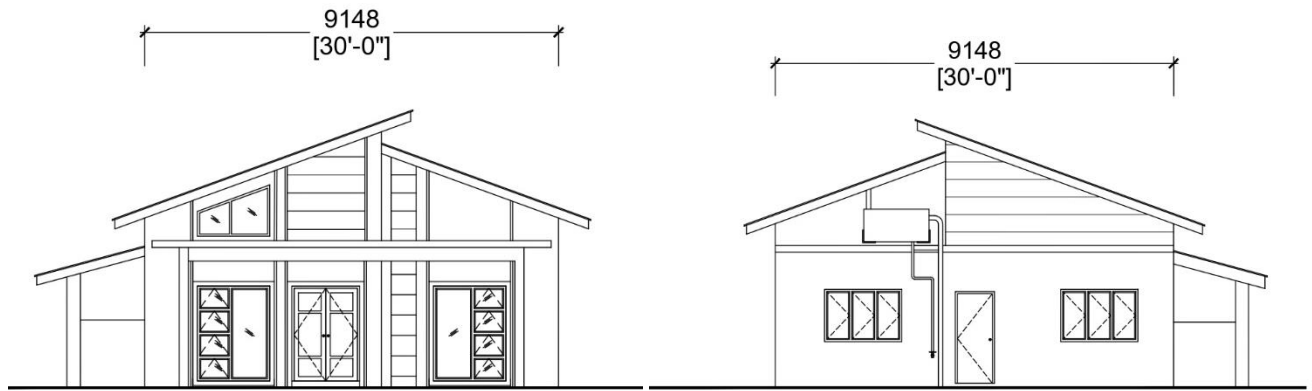
Pandangan Hadapan
