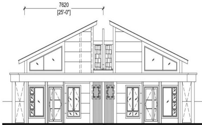
Pandangan Hadapan
