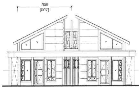
Pandangan Hadapan
