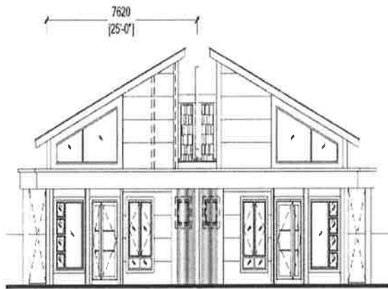
Pandangan Hadapan
