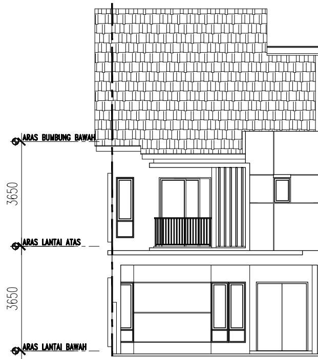
PANDANGAN HADAPAN
