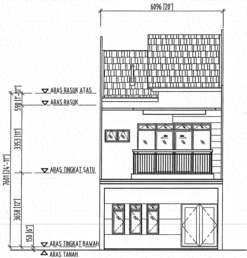
PANDANGAN HADAPAN
