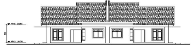
PANDANGAN HADAPAN
