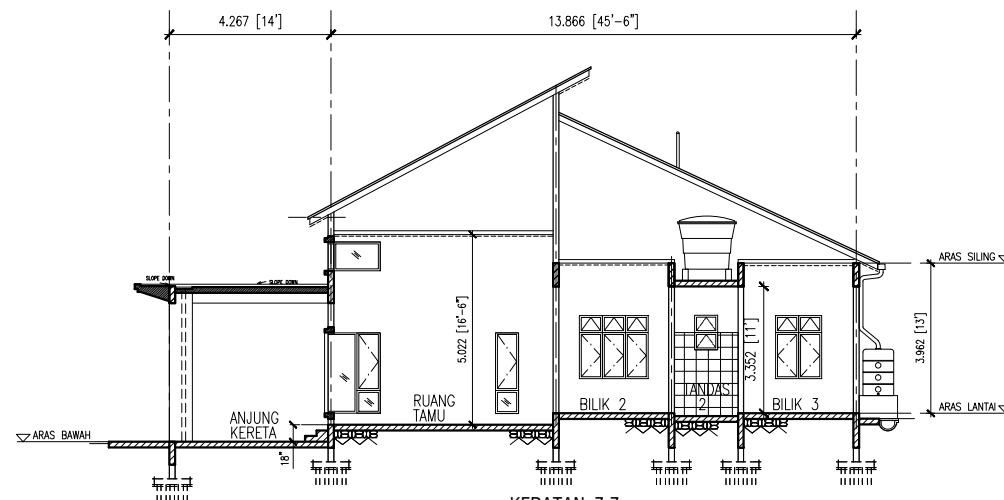
KERATAN Z-Z
