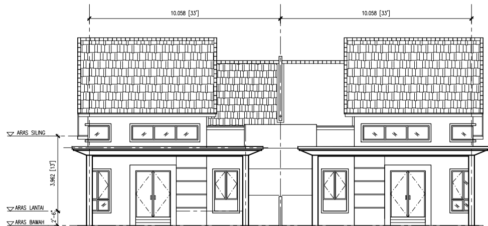
PANDANGAN HADAPAN
