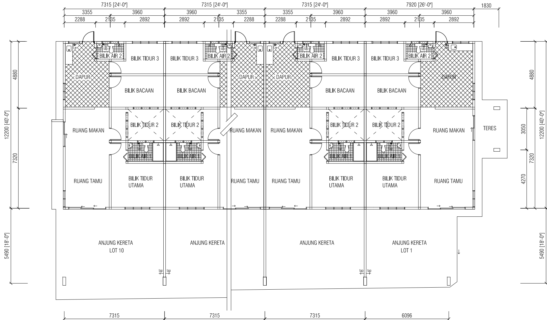
PELAN LANTAI (LOT 1 - 10)
