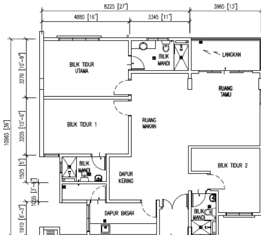
TYPE C3 3 Bilik 1,324 sq.ft
