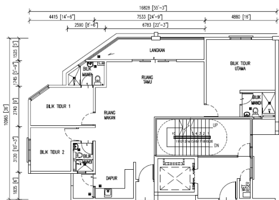
TYPE B2 3 Bilik 1,297 sq.ft
