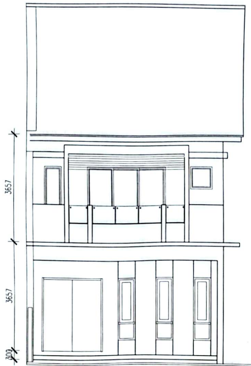
PANDANGAN HADAPAN
