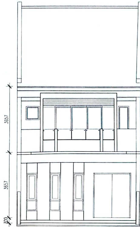
PANDANGAN HADAPAN
