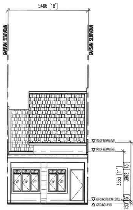
PANDANGAN HADAPAN
