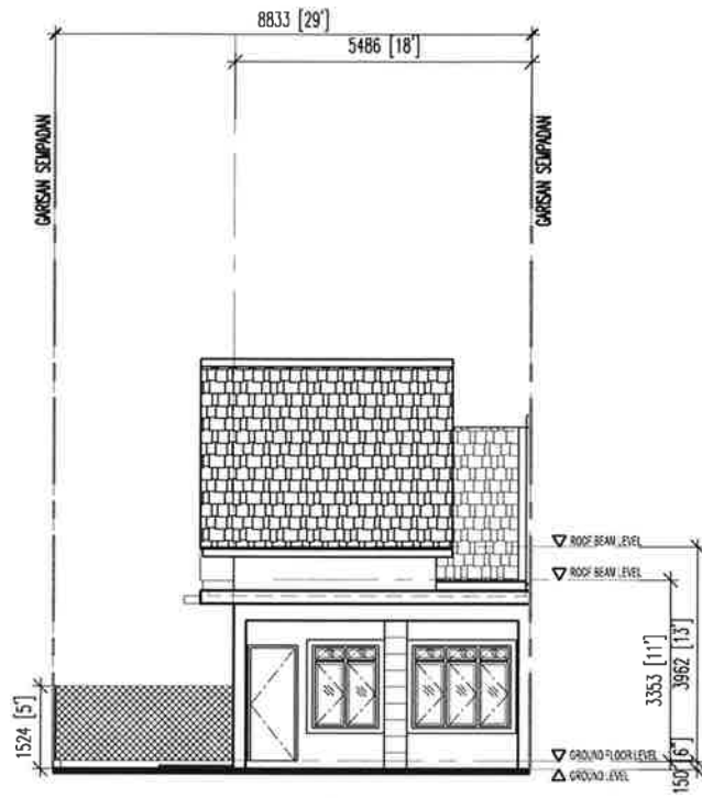
PANDANGAN HADAPAN
