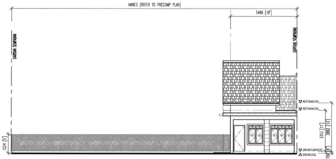
PANDANGAN HADAPAN
