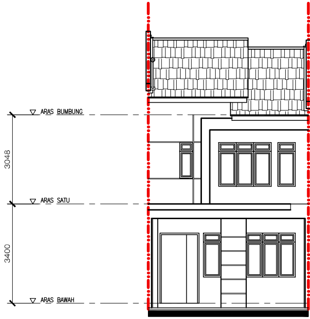
PANDANGAN HADAPAN
