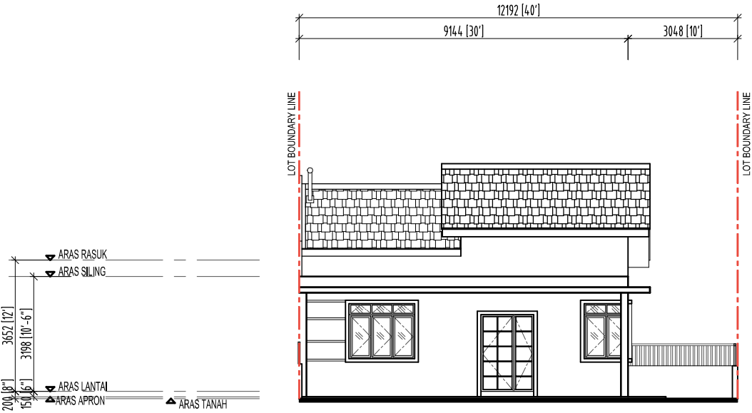
PANDANGAN HADAPAN
