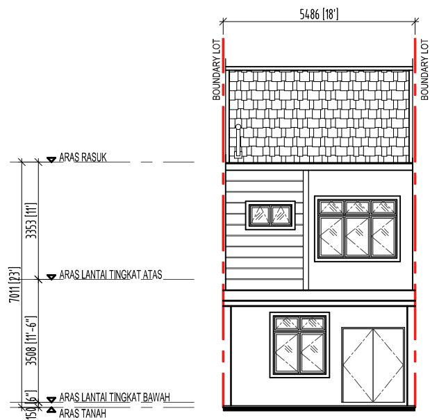
PANDANGAN HADAPAN
