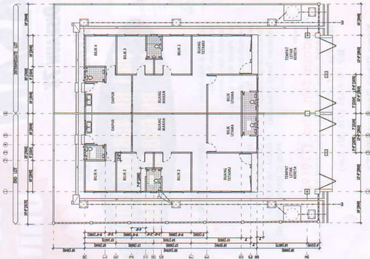
FLOOR PLAN (TYPE 'A')
