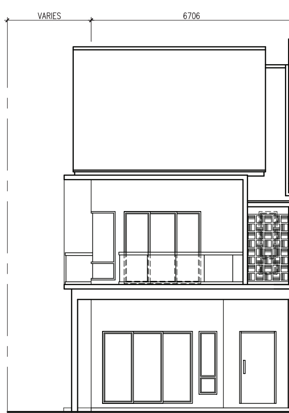
PANDANGAN HADAPAN
