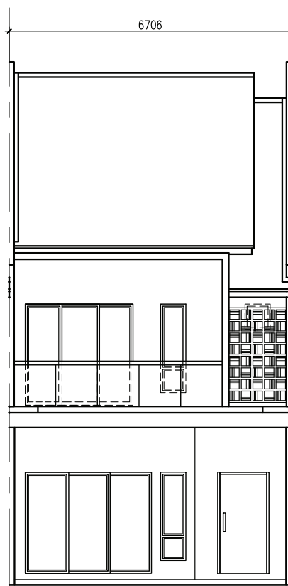
PANDANGAN HADAPAN
