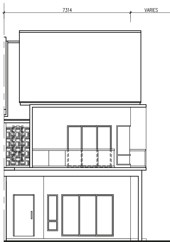
PANDANGAN HADAPAN
