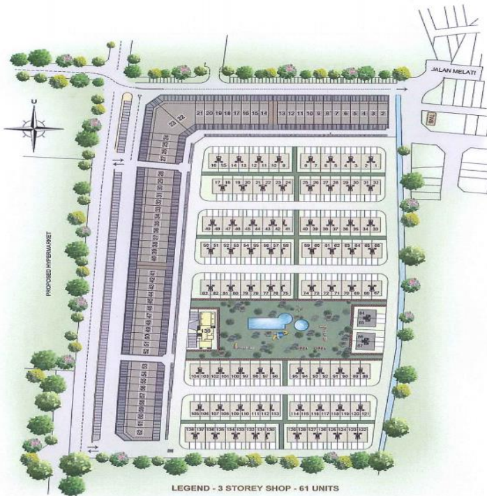
SITE PLAN
