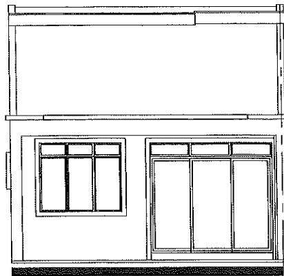
PANDANGAN HADAPAN
