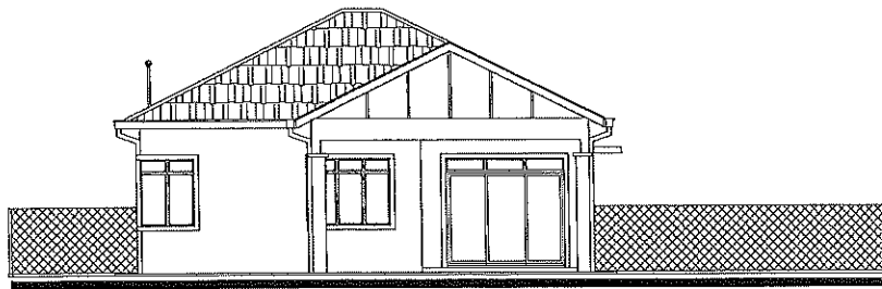
PANDANGAN HADAPAN
