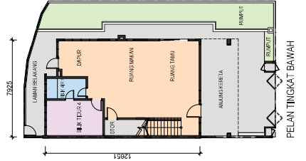
Jenis C 36.5' x 67.5' (3,270 kps)
