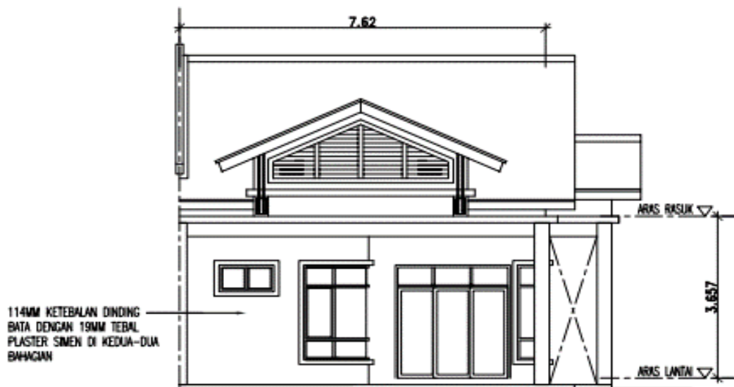
PANDANGAN HADAPAN
