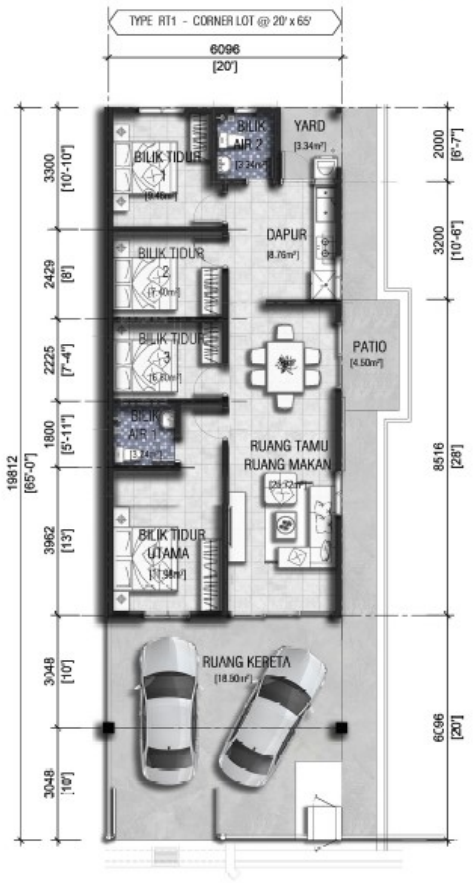
PELAN LANTAI - LOT TEPI
