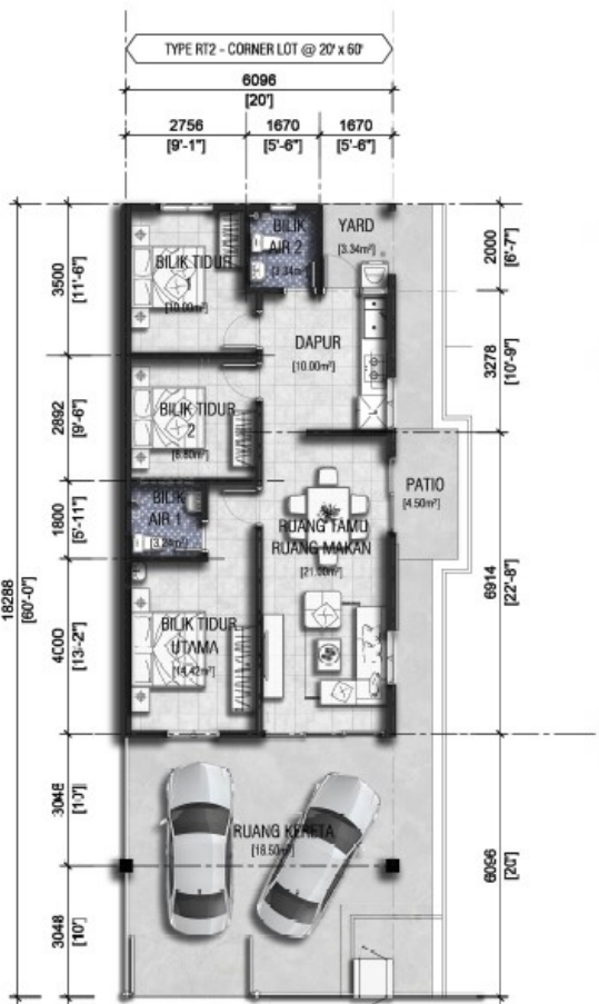
PELAN LANTAI - LOT TEPI
