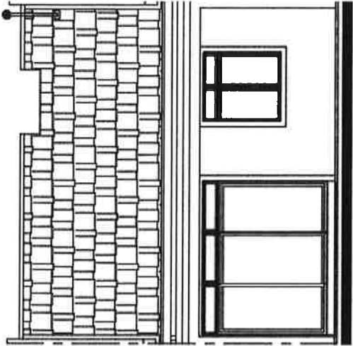
PANDANGAN HADAPAN
