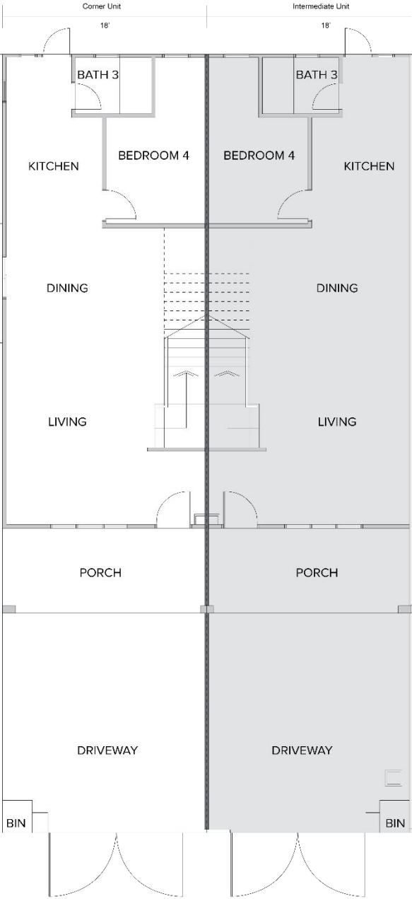
GROUND FLOOR
