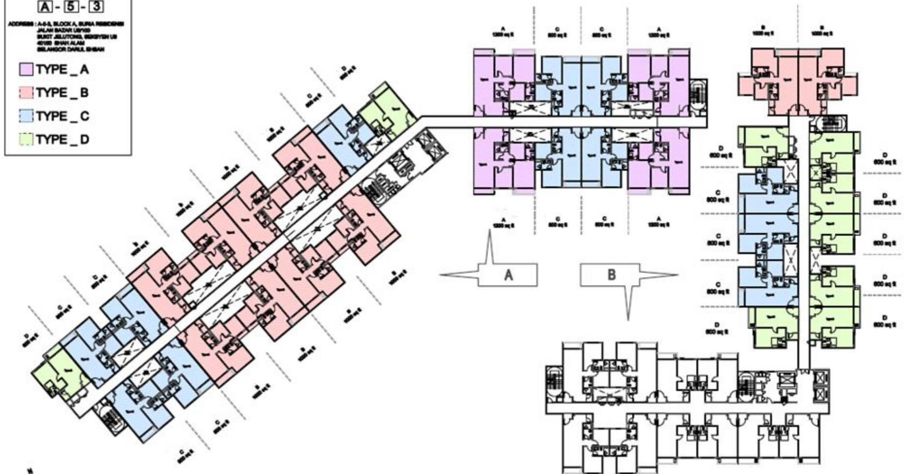
5TH FLOOR PLAN
