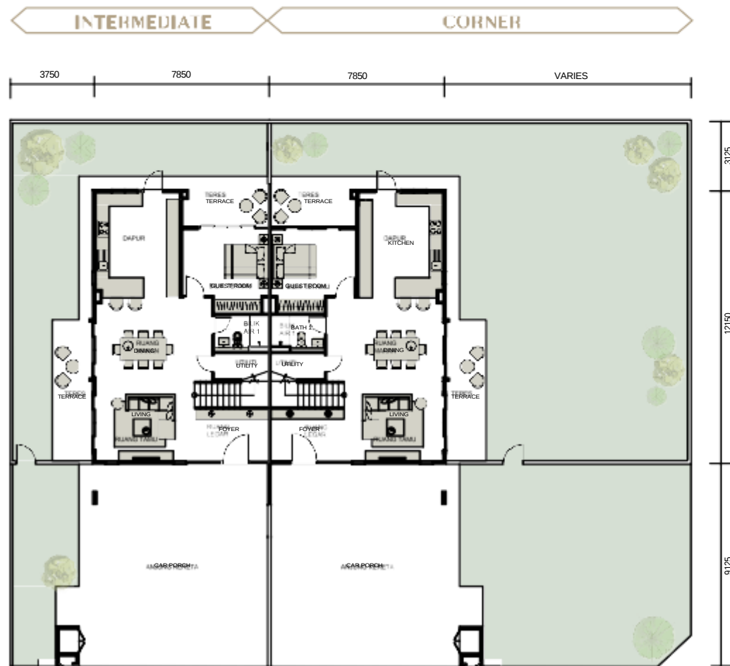
GROUND FLOOR
