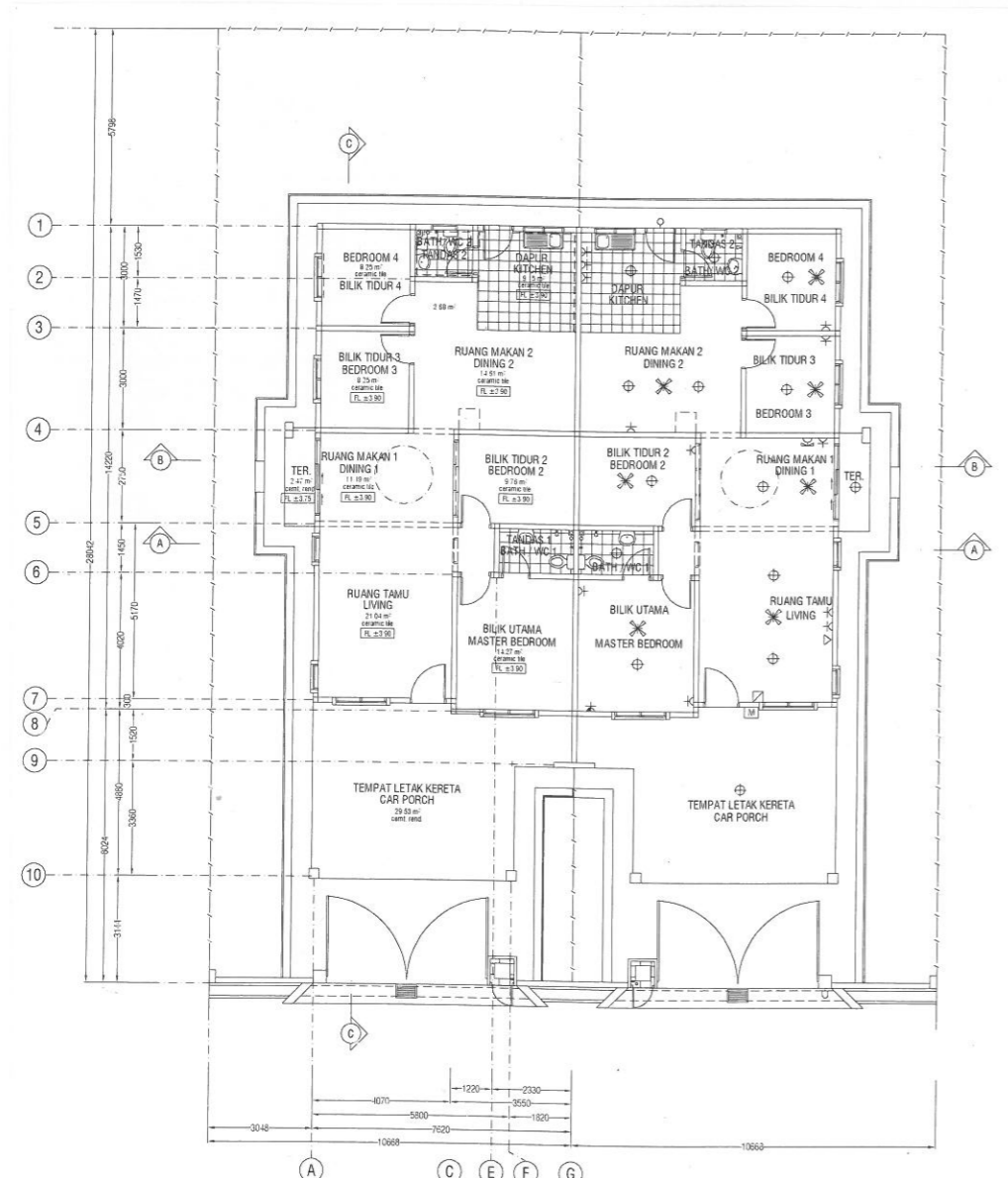
GROUND FLOOR PLAN RUMAH BERKEMBAR SETINGKAT JENIS A & B SCALE: 1:100 ENCLOSED AREA = 107.14 m 2 (1153.24 sq ft) OPEN AREA = 32.00 m 2 (344.44 sq ft) EFFECTIVE BUILT UP AREA = 123.14 m 2 (1325.46 sq ft)
