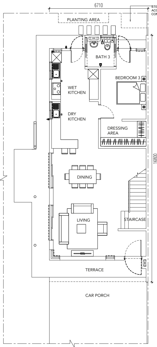
GROUND FLOOR
