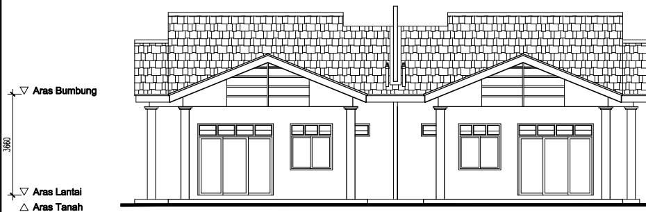
PANDANGAN HADAPAN
