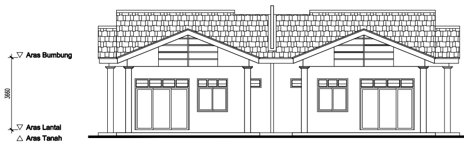
PANDANGAN HADAPAN
