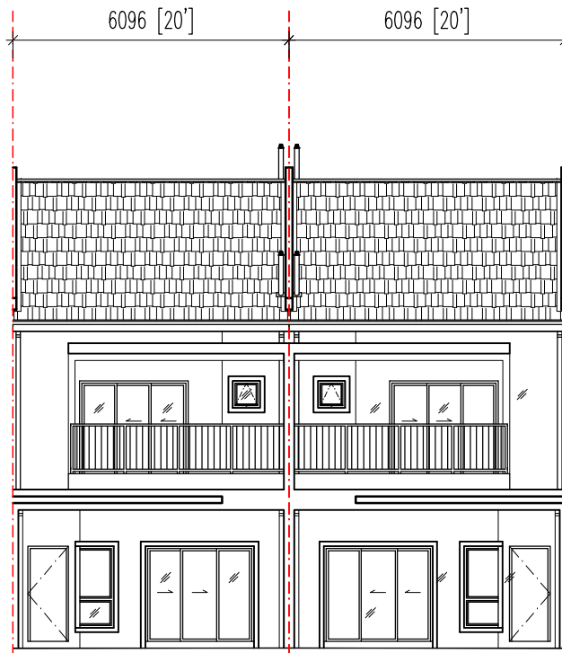
PANDANGAN HADAPAN PT20022, PT20024, PT20026, PT20028, PT20030, PT20033, PT20035, PT20037, PT20039, PT20041
