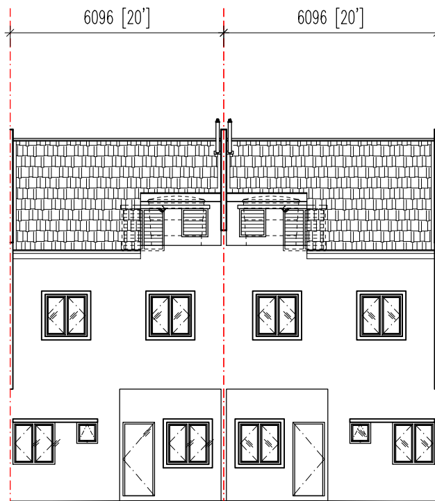
PANDANGAN BELAKANG PT20022, PT20024, PT20026, PT20028, PT20030, PT20033, PT20035, PT20037, PT20039, PT20041
