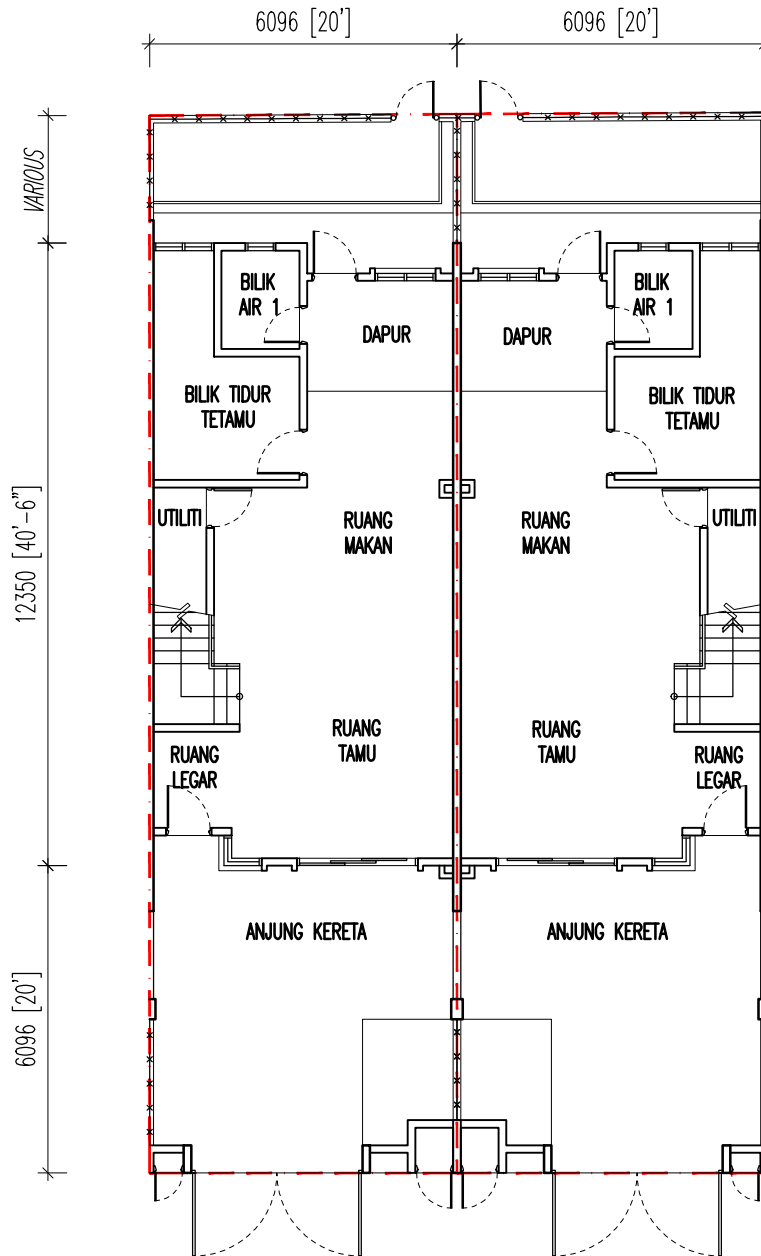
PELAN LANTAI BAWAH PT20022, PT20024, PT20026, PT20028, PT20030, PT20033, PT20035, PT20037, PT20039, PT20041
