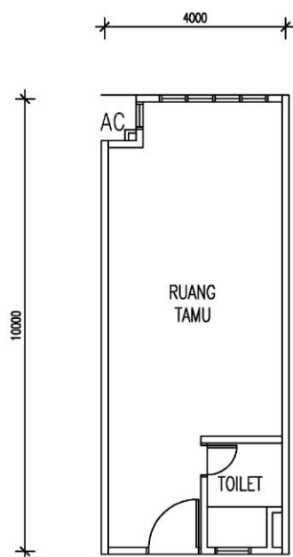
PELAN LANTAI TYPE A3b (intermediate unit) (40.00m 2 / 430.55sqft)
