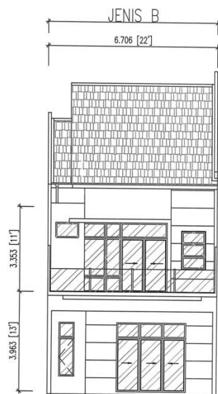
PANDANGAN HADAPAN
