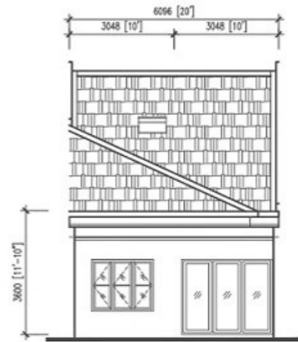
PANDANGAN HADAPAN
