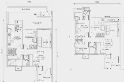
Types A, A1, B, B1, C & C1 Level 8 Built-up area: 1,160 sq. ft. 3 Rooms • 2 Baths
